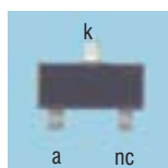
SOT-23 H=1.12, W=3.05, D=2.3
